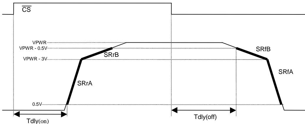
Figure 2. Output Slew Rate and Time Delays
